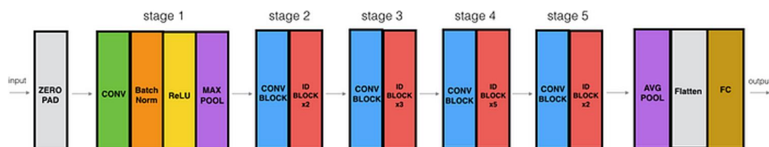
Figure 5. ResNet-50 Architecture
