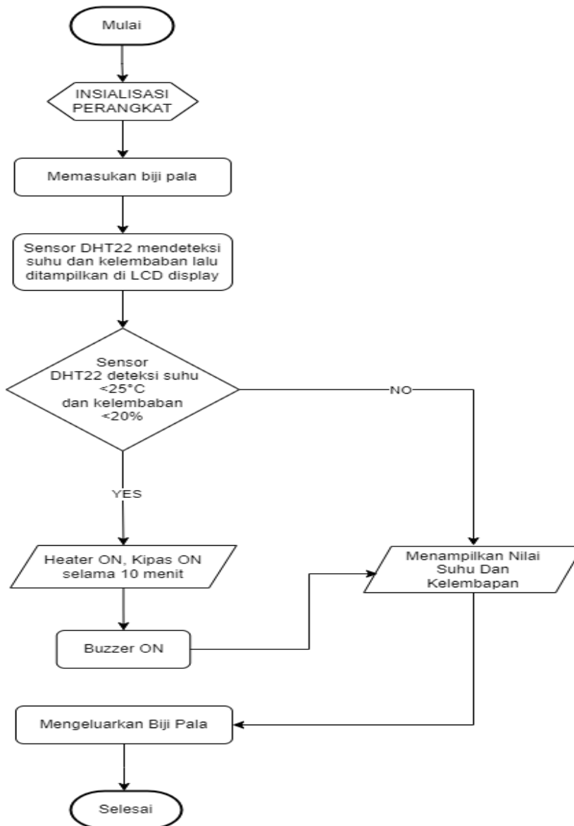
Gambar 4. Flowchart Sistem
